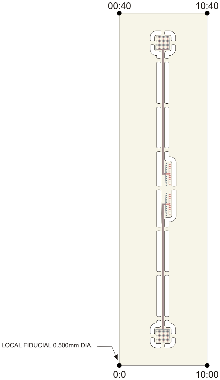
LASER CONTOUR - NESTED PART
