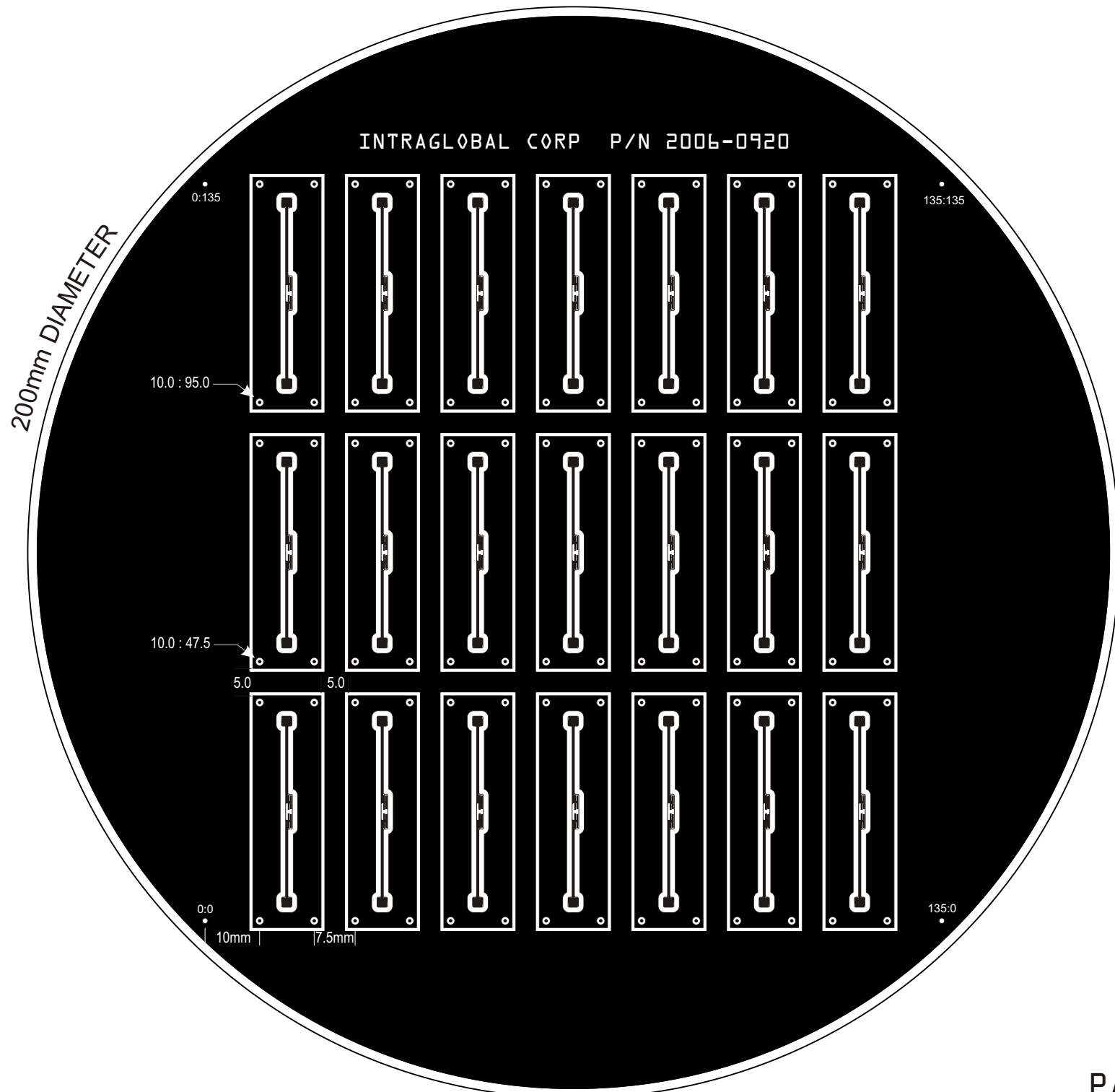
PANEL CONFIG WITH GLOBAL AND LOCAL FIDUCIALS
