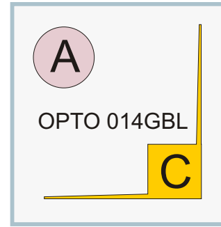
TOP SIDE LOOKING AT THE PADS
