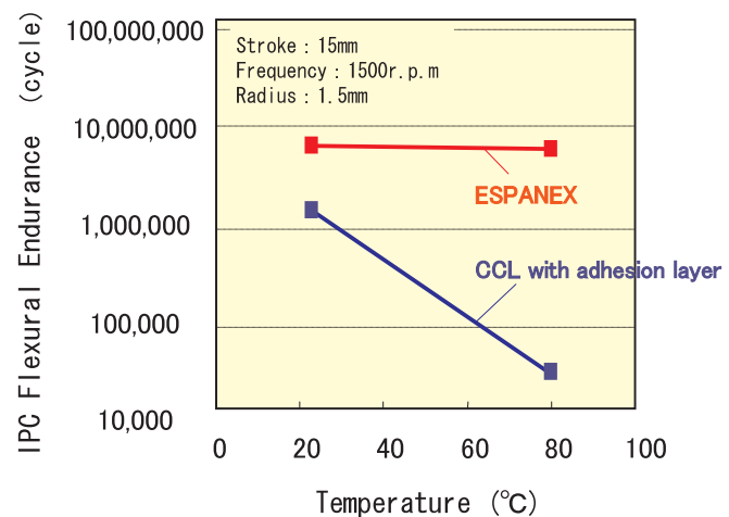
High Temp IPC Flexural Endurance
