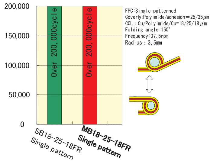
High Temp IPC Flexural Endurance
